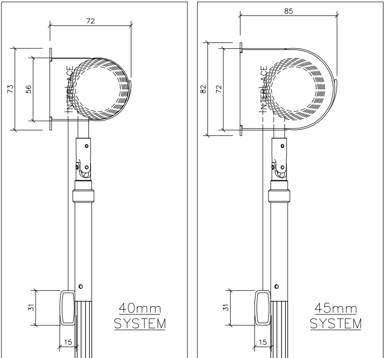
03 FACE FIX CONFIGURATION – SECTION
