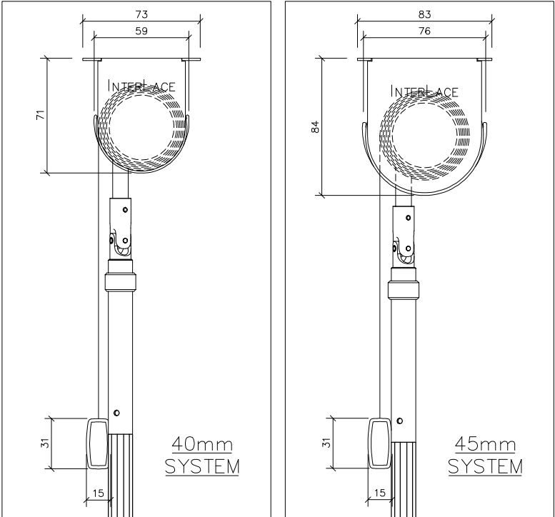
01 TOP FIX CONFIGURATION – SECTION
