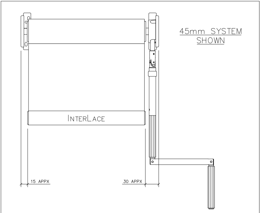
04 FACE FIX CONFIGURATION – ELEVATION
