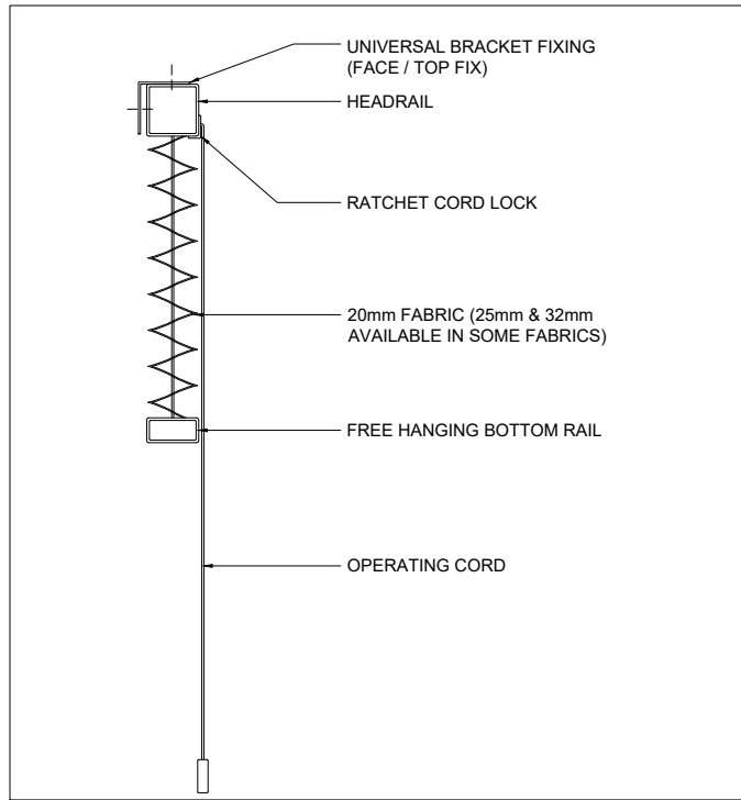
03 - SECTION - BLIND PART LOWERED
