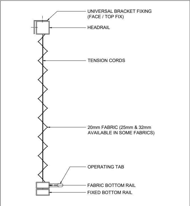
01 - SECTION - BLIND LOWERED
