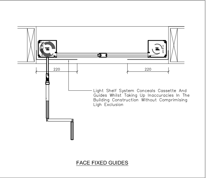
04 - LIGHT SHELF OPTION
