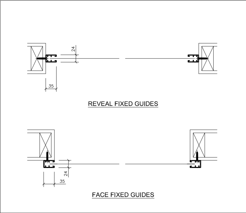
03 - SECTIONS THROUGH GUIDES
