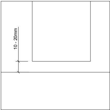
FLOOR CLEARANCE
