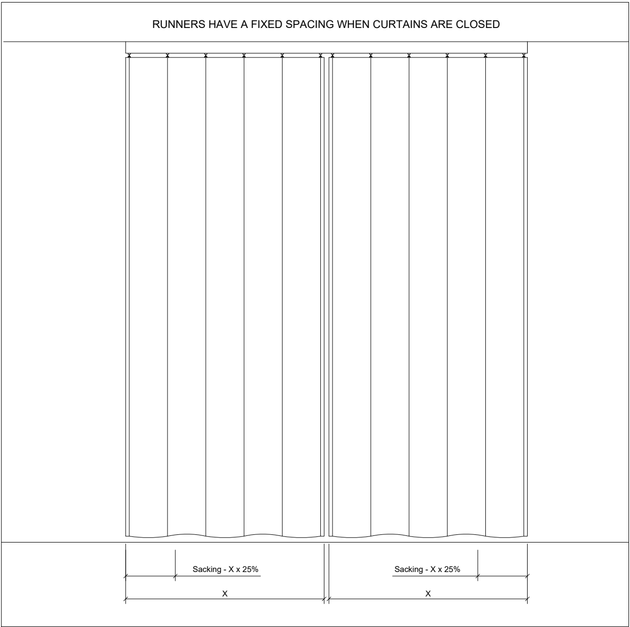
02 - TYPICAL ELEVATION
