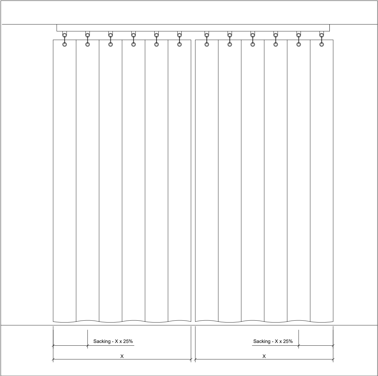
02 - TYPICAL ELEVATION
