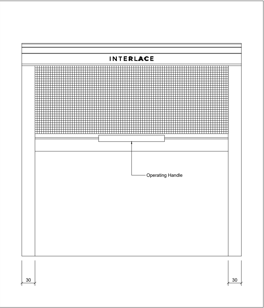
02 - TYPICAL ELEVATIONS
