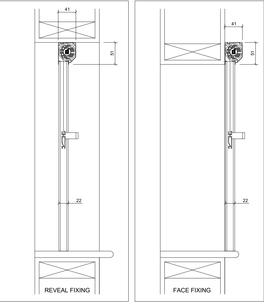
01 - SECTIONS
