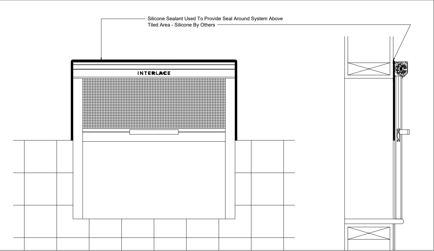
04 - FIXING TO PART TILED WALL
