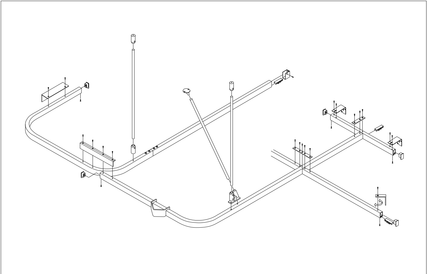
02 - TYPICAL EXPLODED VIEW
