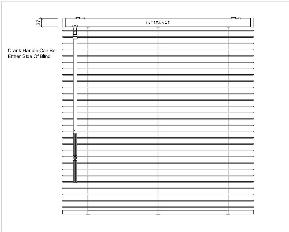
04 - TYPICAL ELEVATION - 35mm SLAT
