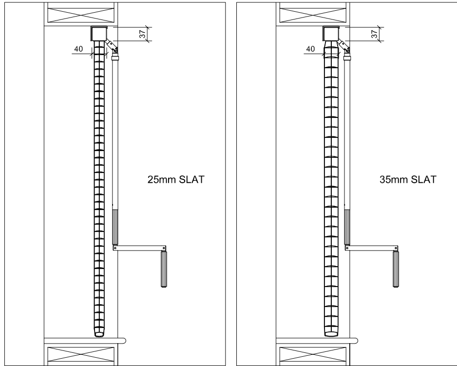
01 - TOP FIX CONFIGURATION - SECTION
