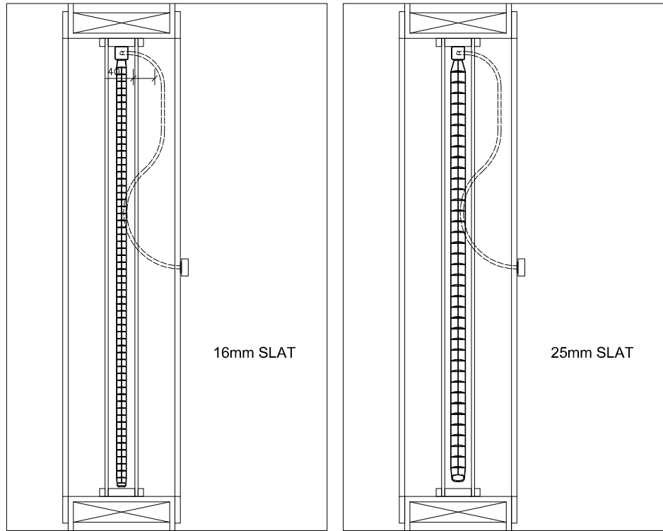
01 - SECTION - KNB TILT CONTROL
