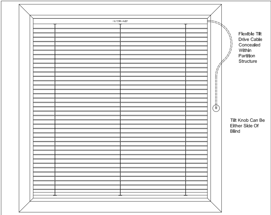
03 - TYPICAL ELEVATION - 25mm SLAT
