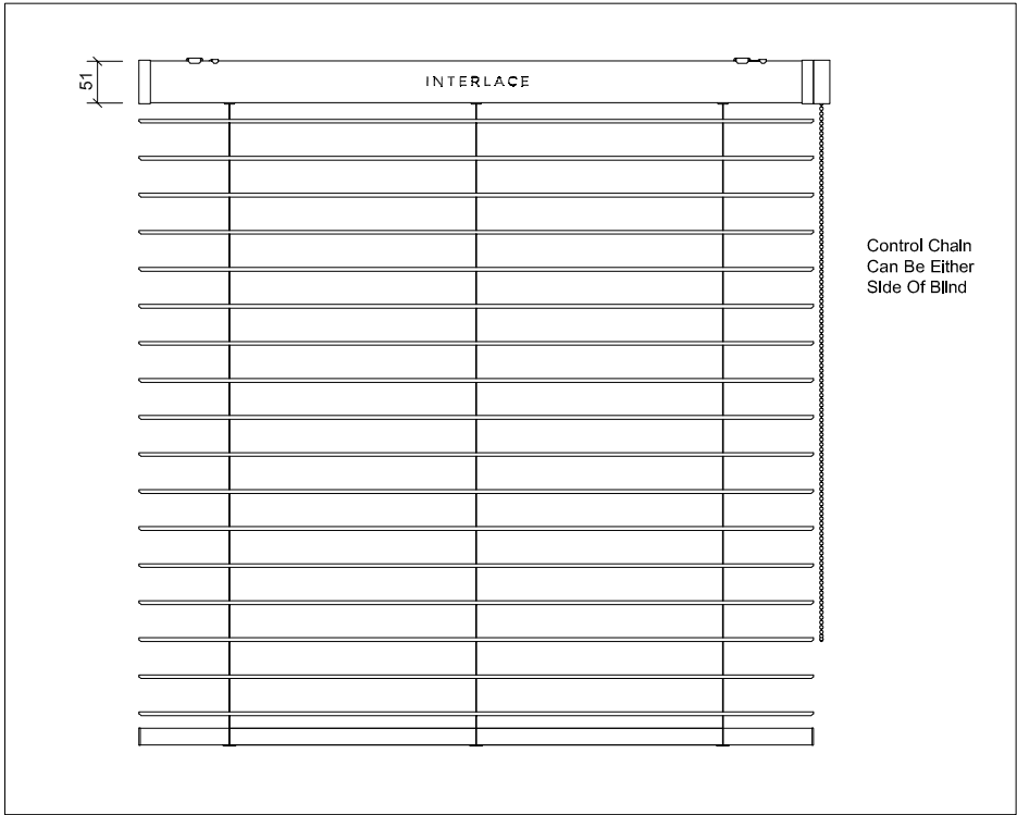
04 - TYPICAL ELEVATION - 50mm SLAT
