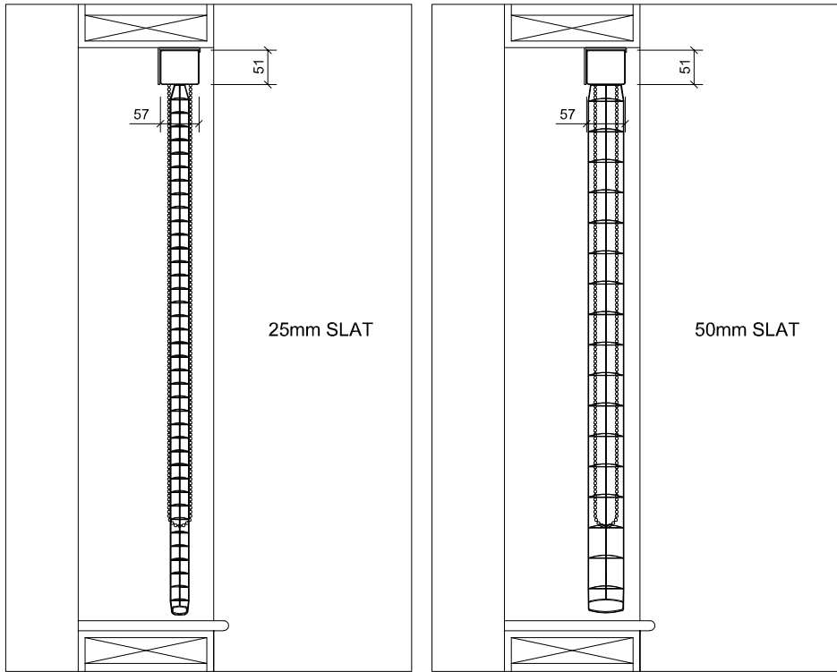
01 - TOP FIX CONFIGURATION - SECTION
