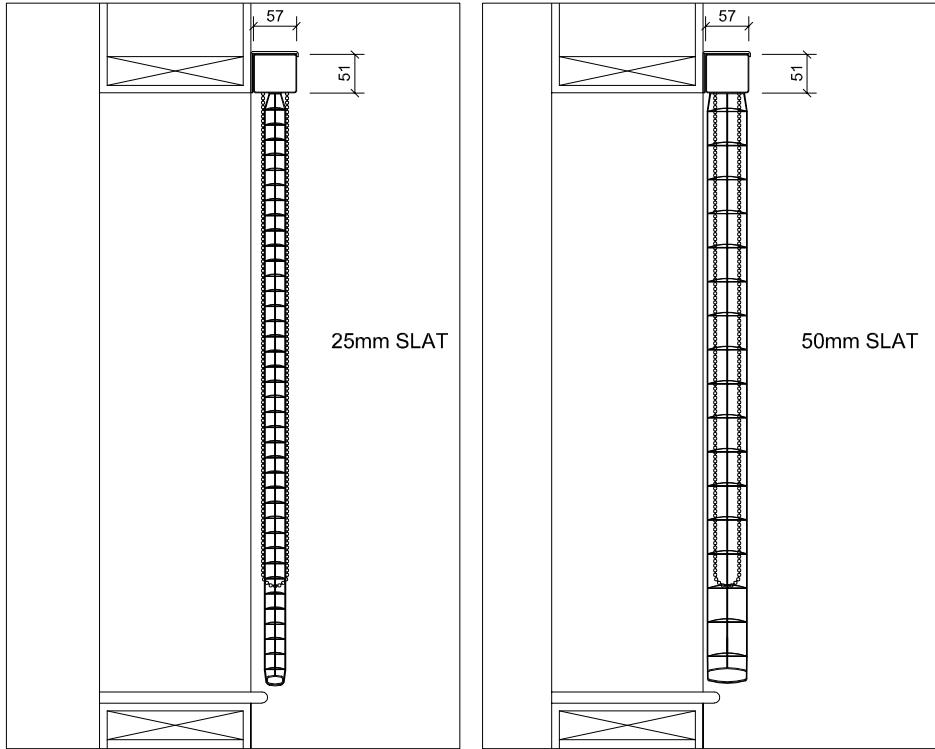
03 - FACE FIX CONFIGURATION - SECTION
