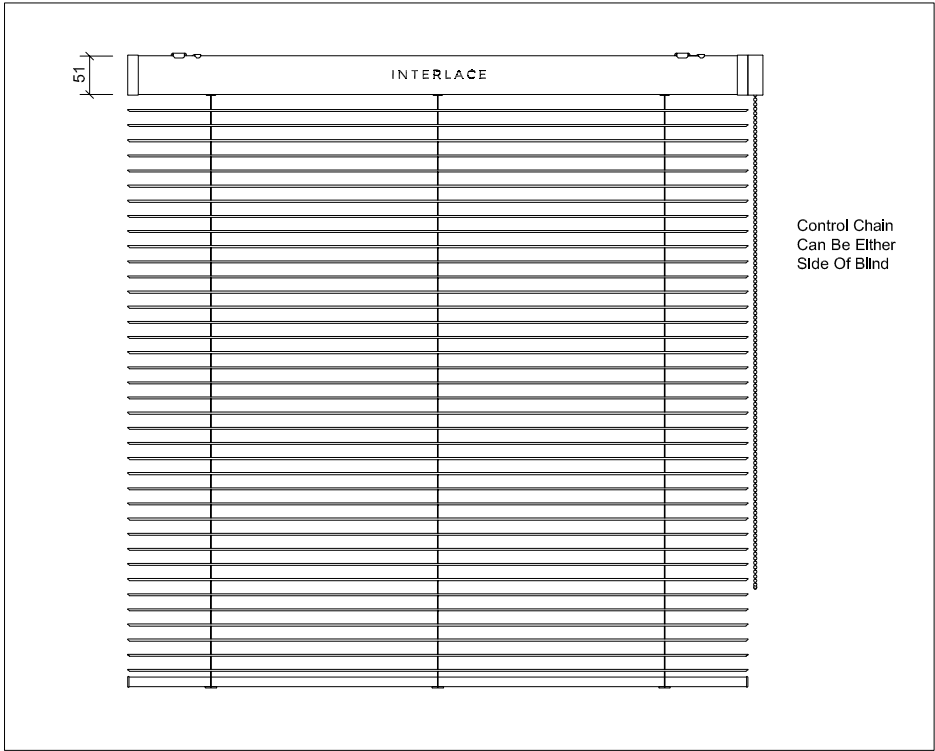
02 - TYPICAL ELEVATION - 25mm SLAT
