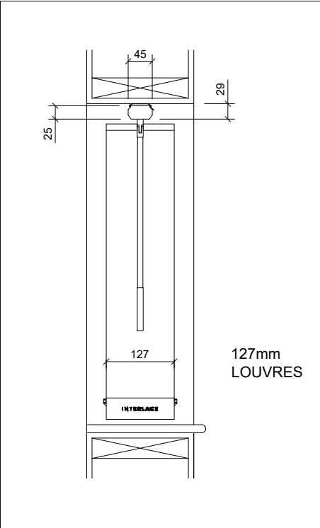
01 - SECTION - REVEAL FIXING
