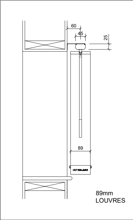
02 - SECTION - FACE FIXING
