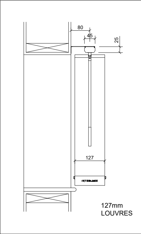
04 - TYPICAL ELEVATION - 127mm LOUVRES
