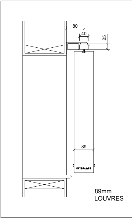
03 - SECTION - FACE FIXING
