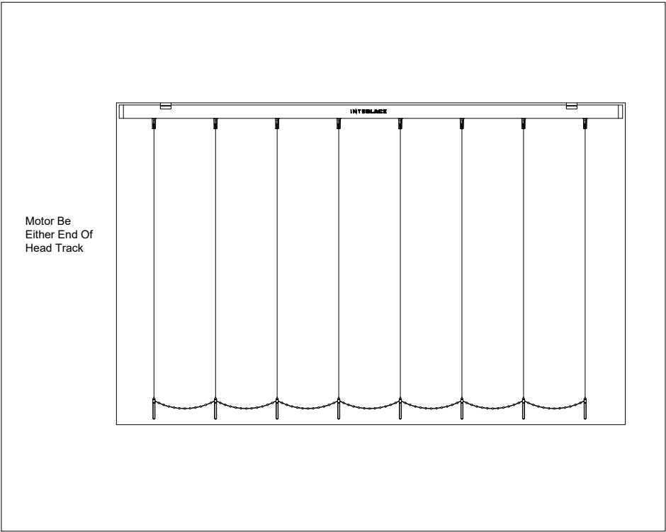
04 - TYPICAL ELEVATION - 127mm LOUVRES
