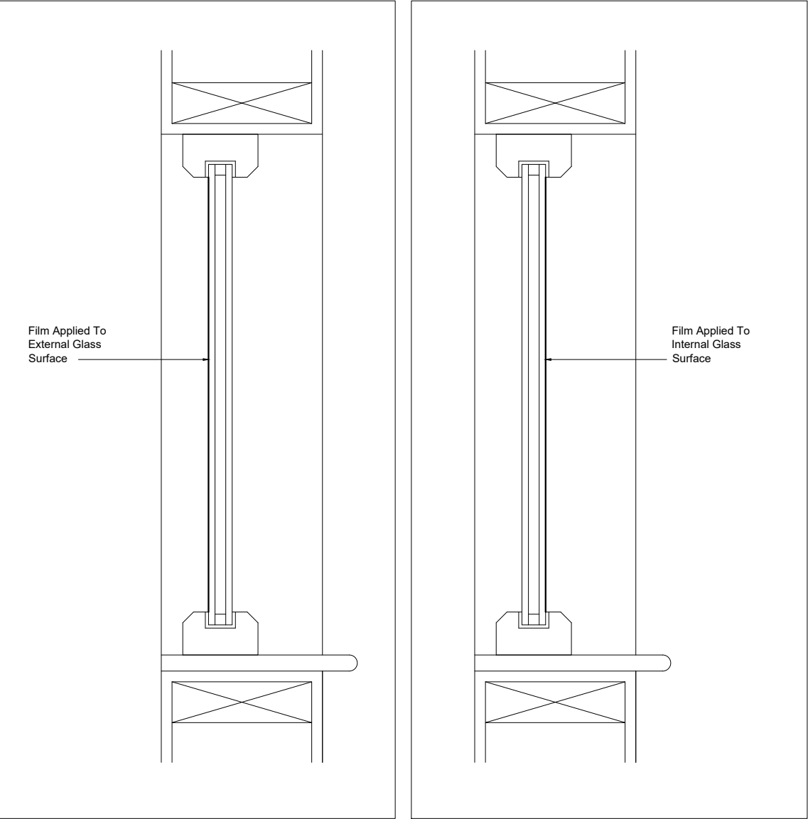
01 - SECTIONS
